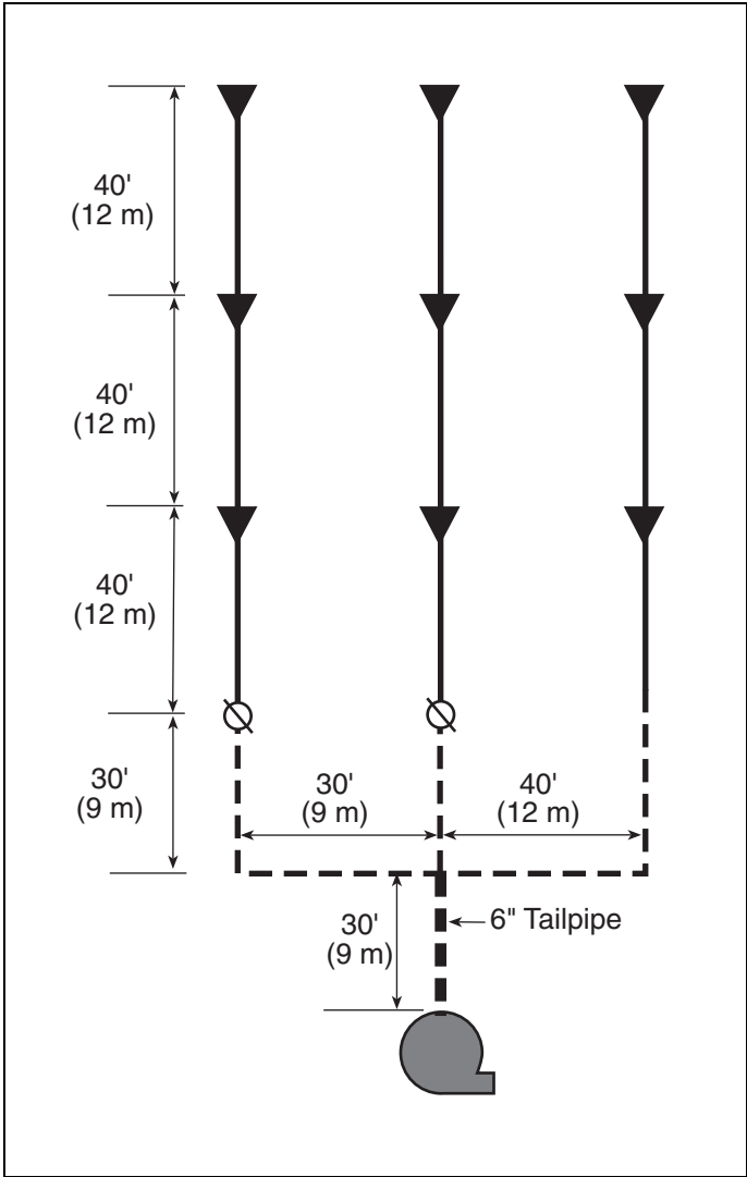
FIGURE 21: Example System Layout (Option 4)
